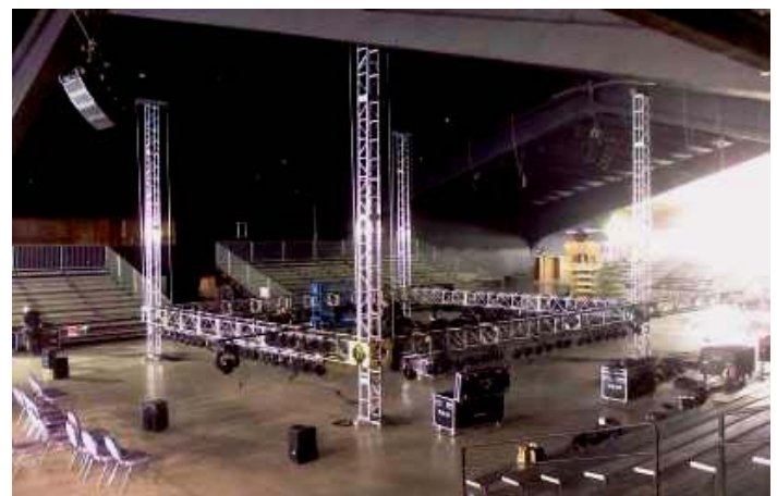
Figure 2: Typical ground support temporary structure
